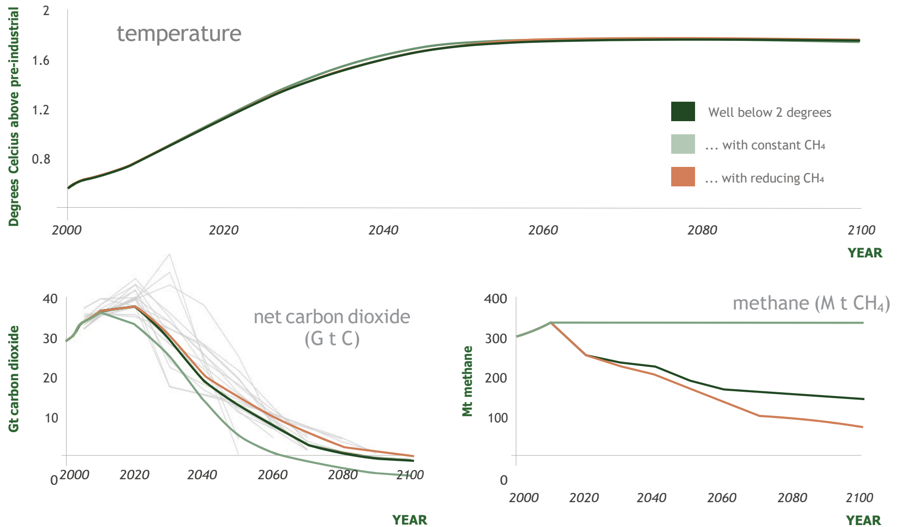
Figure 6: Three alternative scenarios for global emissions of carbon dioxide and methane that limit the temperature rise to 2°C
