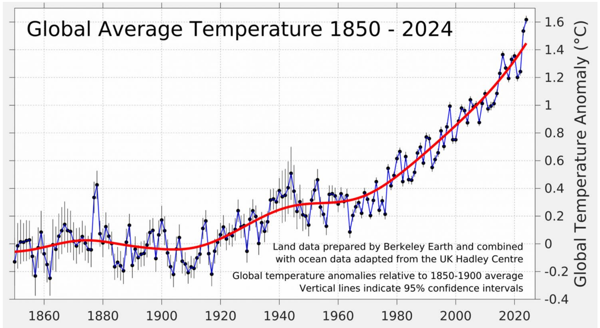
Figure 3: Global Average Temperature 1850-2024
