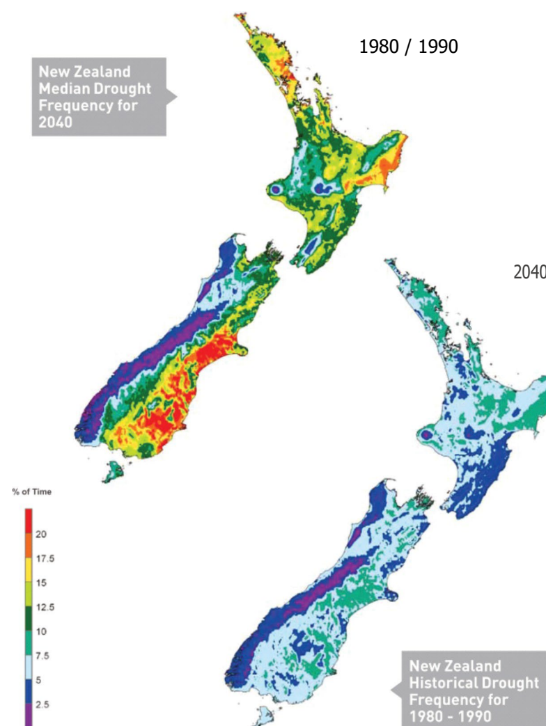
Figure 2: NZ median drought frequency for 1980/90 and 2040
